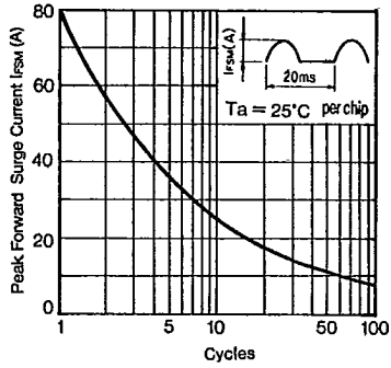
IFSM Characteristics
