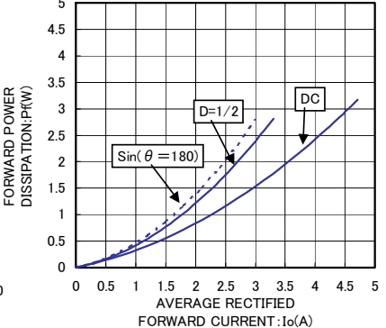
Io-Pf CHARACTERISTICS
