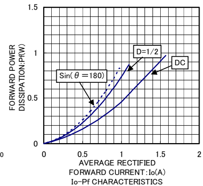
Io-Pf CHARACTERISTICS
