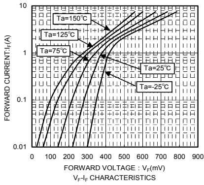
V_F - I_F CHARACTERISTICS
