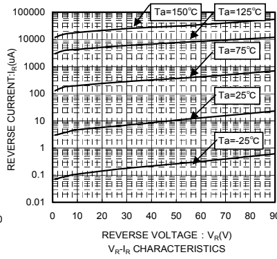
V_R - I_R CHARACTERISTICS
