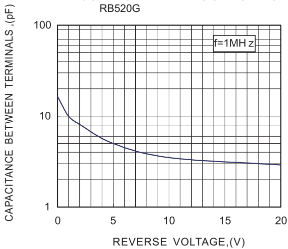
FIG.3-TYPICAL TERMINALS CAPACITANCE RB520G
