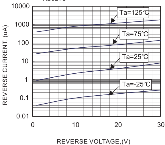
FIG.2 - TYPICAL REVERSE CHARACTERISTICS RB521G
