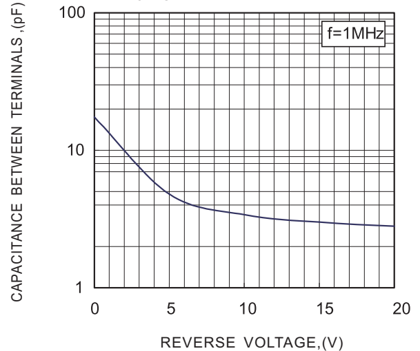
FIG.3-TYPICAL TERMINALS CAPACITANCE RB521G
