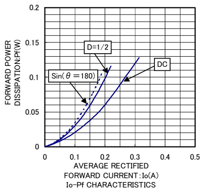
Io-Pf CHARACTERISTICS
