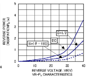
VR-Prr CHARACTERISTICS
