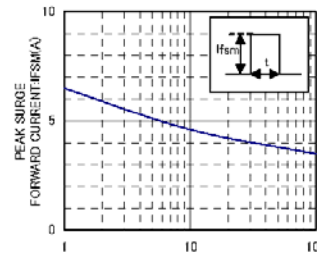
IFSM-t CHARACTERISTICS
