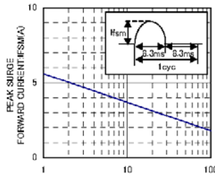
IFSM-CYCLE CHARACTERISTICS
