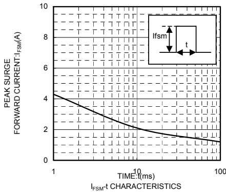
I_{FSM}-t CHARACTERISTICS
