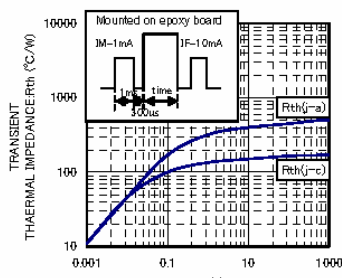
TIME: t(s) Rth-t CHARACTERISTICS
