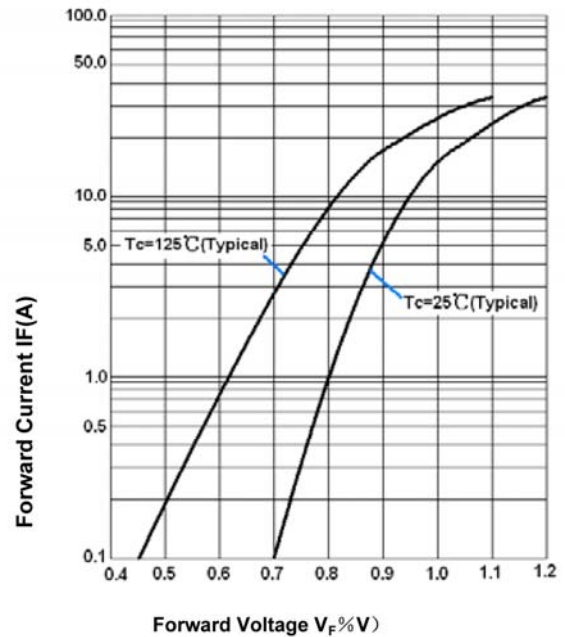
Fig.4 Forward Voltage
