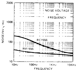
Noise Voltage
