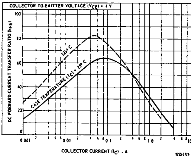
Fig. 7 - Typical dc beta characteristics for RCA3054.
