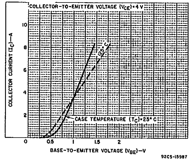
Fig. 10 — Typical transfer characteristics for RCA3055.
