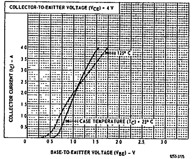
Fig. 6 - Typical transfer characteristics for RCA3054.
