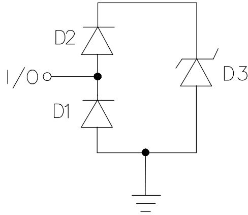
Figure 1 - RClamp0504P Spice Model
