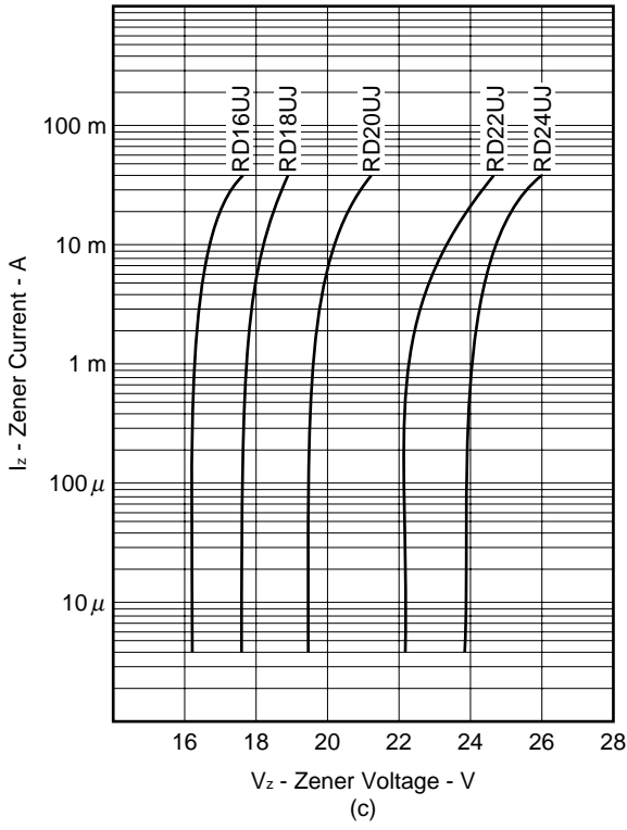
Fig. 3 \gamma_z - V_z CHARACTERISTICS
