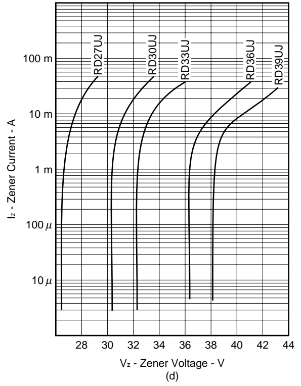
Fig. 3 \gamma_z - V_z CHARACTERISTICS
