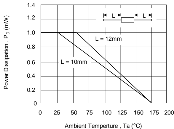
Fig. 1 Derating Curve
