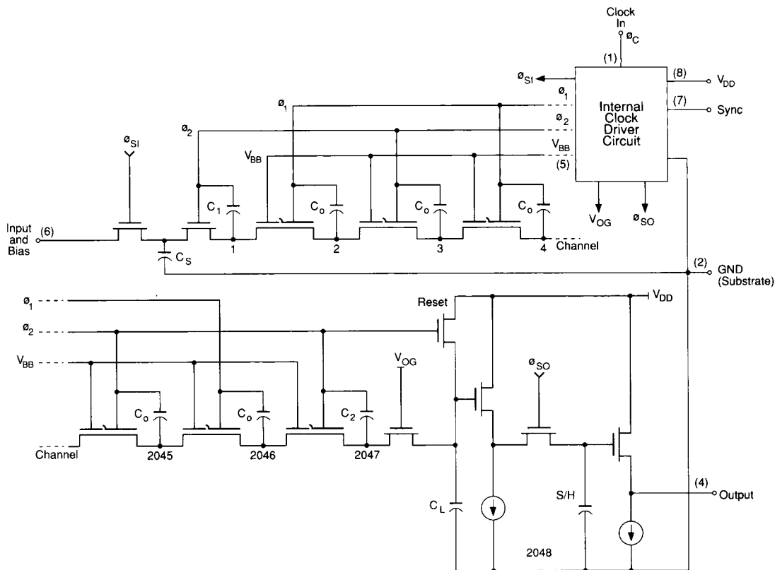
Figure 2. Equivalent Circuit
