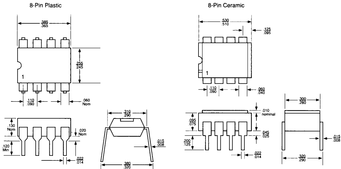
Figure 9. Package Dimensions
