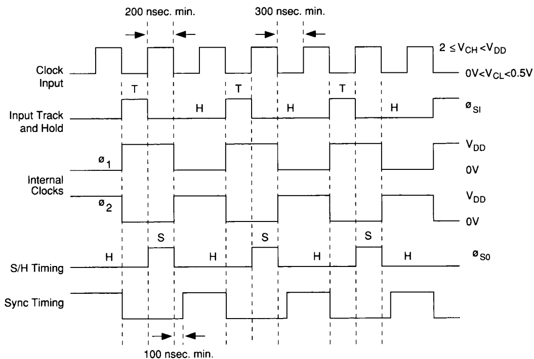
Figure 4. Timing Relations
