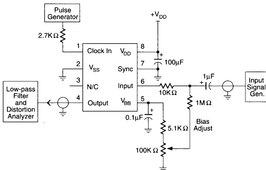
Figure 3. Test Configuration
