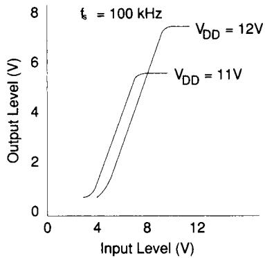
Figure 5. Typical DC Output vs. DC Input
