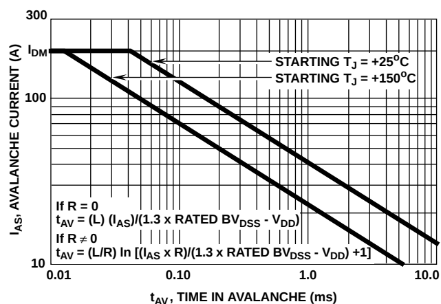
FIGURE 2. UNCLAMPED INDUCTIVE-SWITCHING
