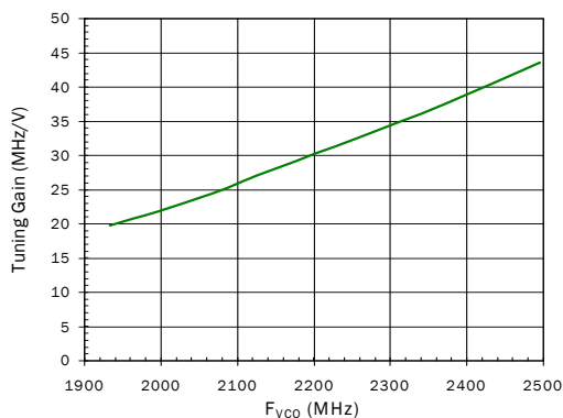
VC02 Tuning Gain versus Frequency
