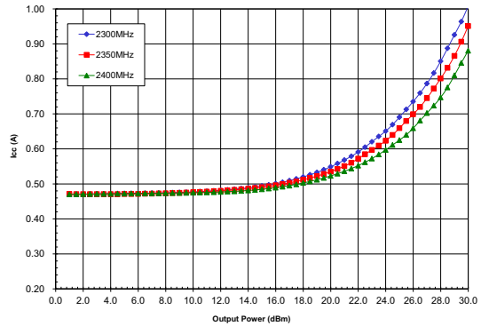
Icc(A) vs. Pout(dBm) 85° C Vcc=5Vdc Vreg=5Vdc
