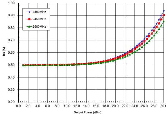
Icc(A) vs. Pout(dBm) 25° C Vcc=5Vdc Vreg=5Vdc
