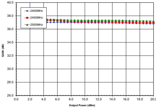
Gain(dB) vs. Pout(dBm) 85° C Vcc=5Vdc Vreg=5Vdc
