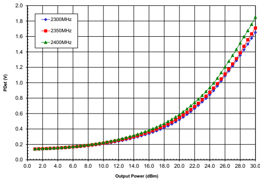
Power Detect (V) vs. Pout(dBm) 25° C Vcc=5Vdc Vreg=5Vdc
