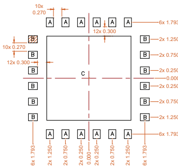
PCB METAL LAND PATTERN
