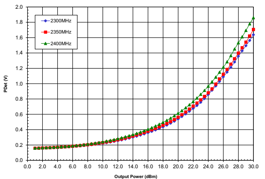
Power Detect (V) vs. Pout(dBm) 85° C Vcc=5Vdc Vreg=5Vdc
