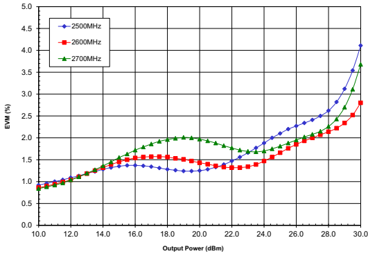
EVM(%) vs. Pout(dBm) 85° C Vcc=5Vdc Vreg=5Vdc
