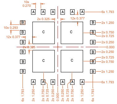
PCB STENCIL PATTERN
