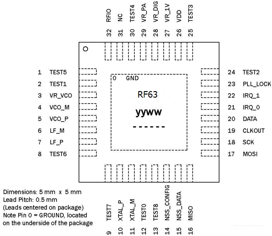
Figure 2: RF63 Pin Diagram
