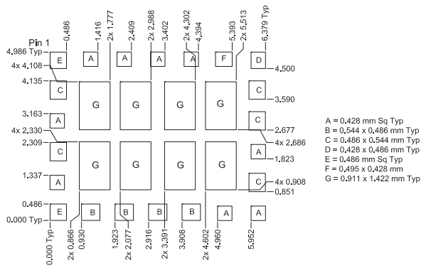
PCB STENCIL PATTERN
