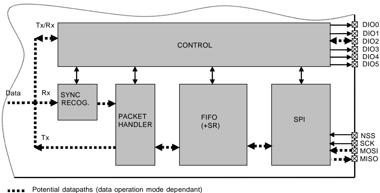
Figure 31. RF92/93 Data Processing Conceptual View
