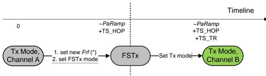
Figure 28. Transmitter Hopping
