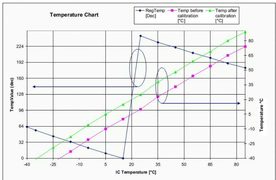
Figure 9. Temperature Sensor Response
