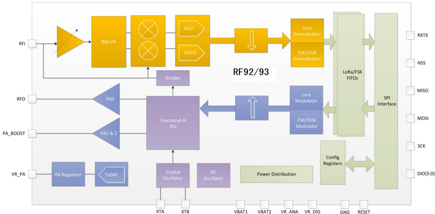
Figure 1. Block Diagram
