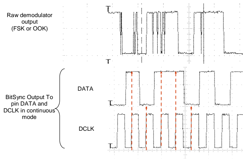
Figure 21. Bit Synchronizer Description
