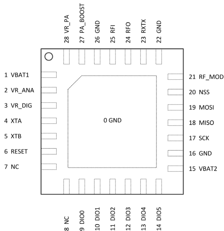
Figure 2. Pin Diagram
