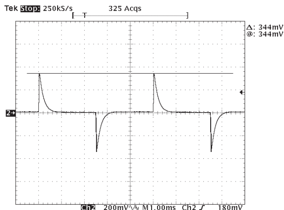
Figure 11 - RFF600-24S28Y Transient Response Load 10.70 A to 16.05 A
