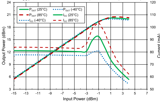
P OUT and Current versus Input Power (150MHz)
