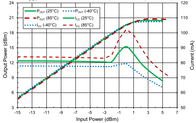
P OUT and Current versus Input Power (450MHz)
