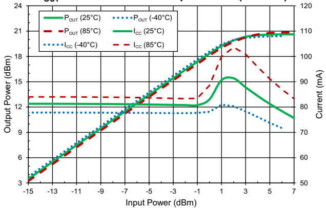
P OUT and Current versus Input Power (850MHz)
