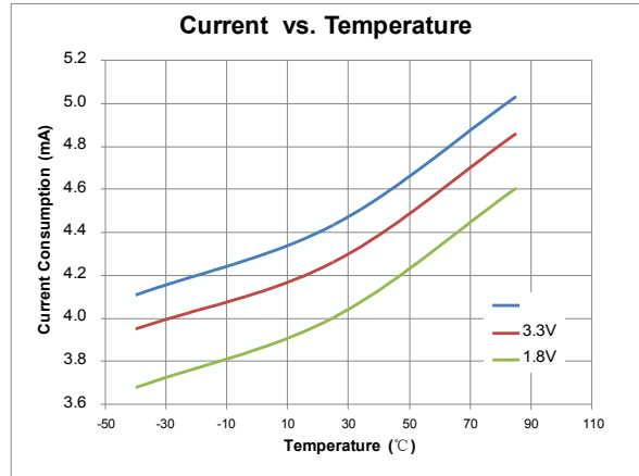
Figure 4. Current vs. Temperature, F_{RF} = 433.92 MHz, FSK, SR = 1 kbps
