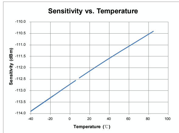
Figure 6. Sensitivity vs. Temperature, F_{RF} = 433.92 MHz, V_{DD} = 3.3 V, SR = 1 kbps, FSK, BER = 0.1%
