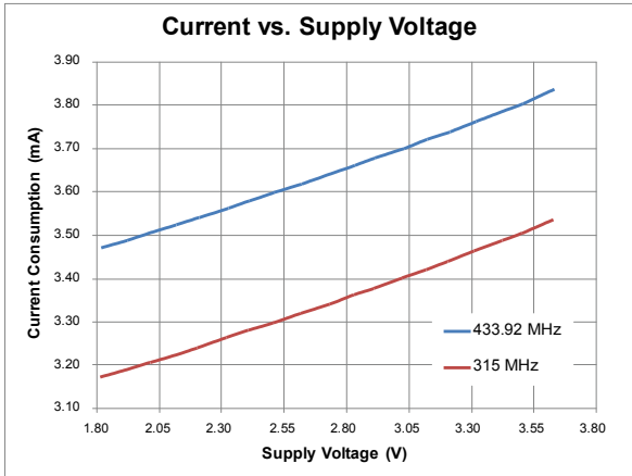
Figure 3. Current vs. Voltage, F_{RF} = 315 / 433.92 MHz, OOK, SR = 1 kbps
