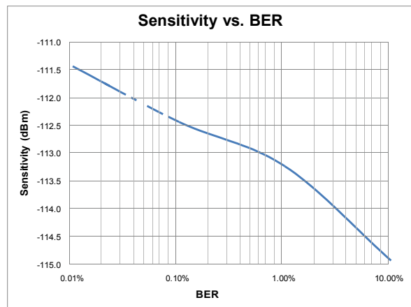
Figure 8. Sensitivity vs. BER, F_{RF} = 433.92 MHz, V_{DD} = 3.3 V, SR = 1 kbps, FSK
