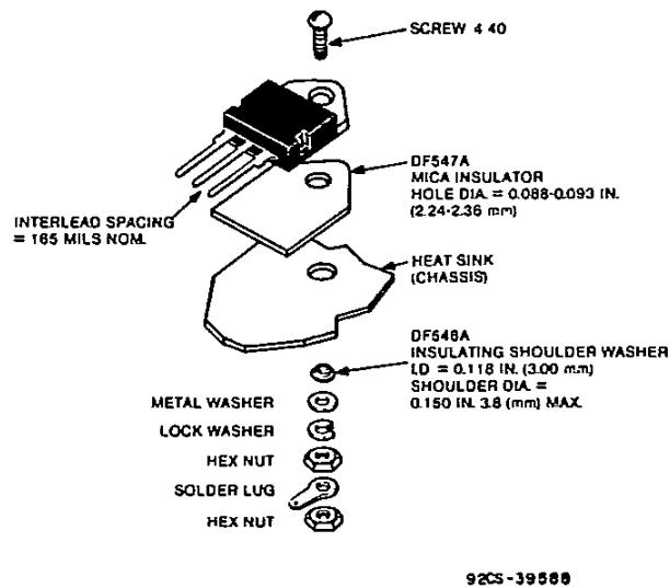
Suggested mounting hardware for JEDEC TO-218AC
