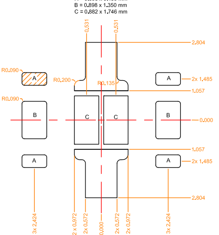
PCB STENCIL PATTERN
