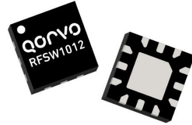
12 Pin 2 mm x 2 mm leadless QFN Package
