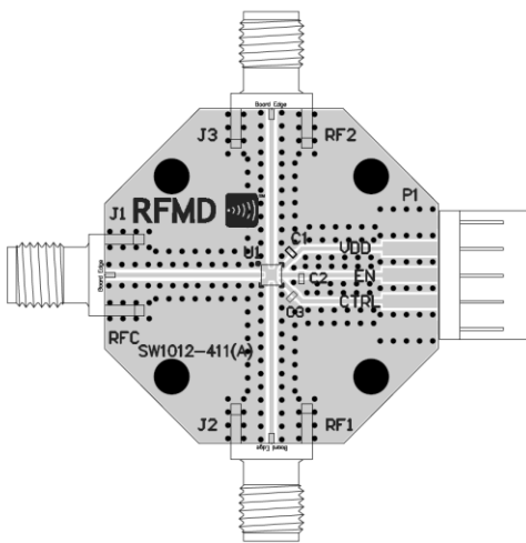
50Ω Evaluation Board
