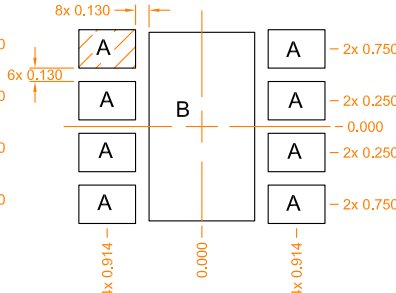
PCB SOLDER MASK PATTERN
