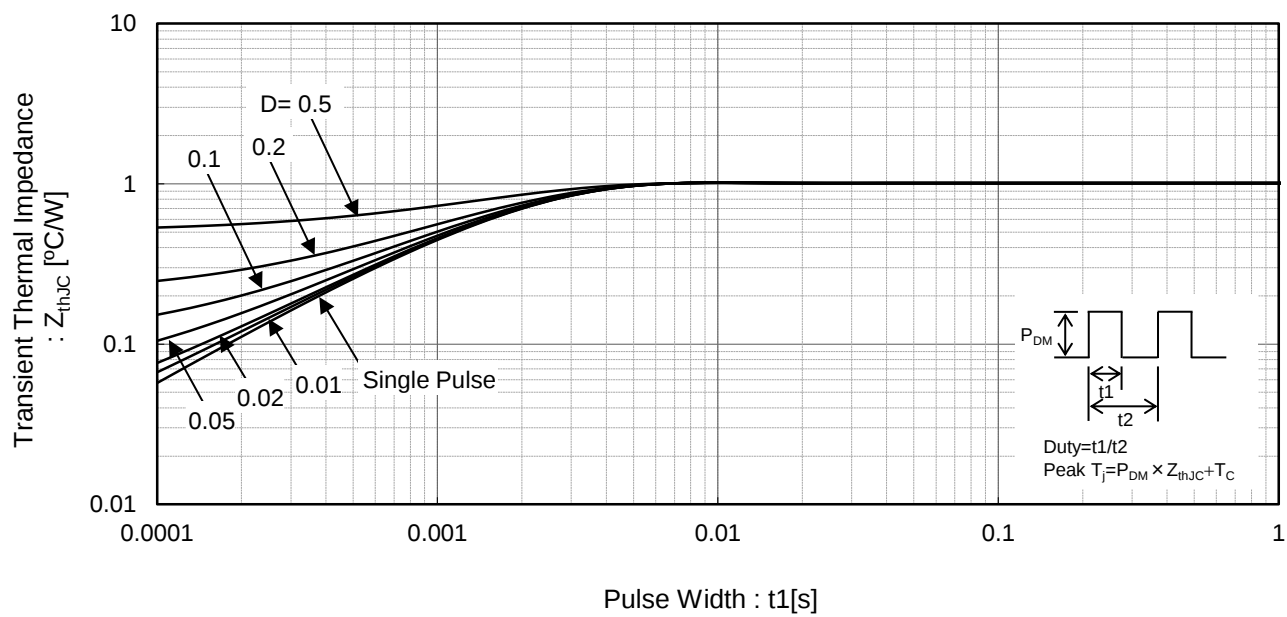
Fig.17 IGBT Transient Thermal Impedance
