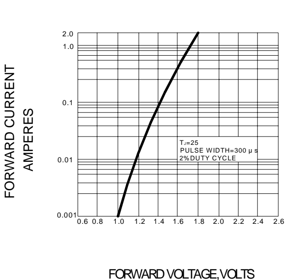
FIG.4–TYPICAL FORWARD CHARACTERISTIC
