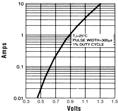
Typical Instantaneous Forward Characteristics
