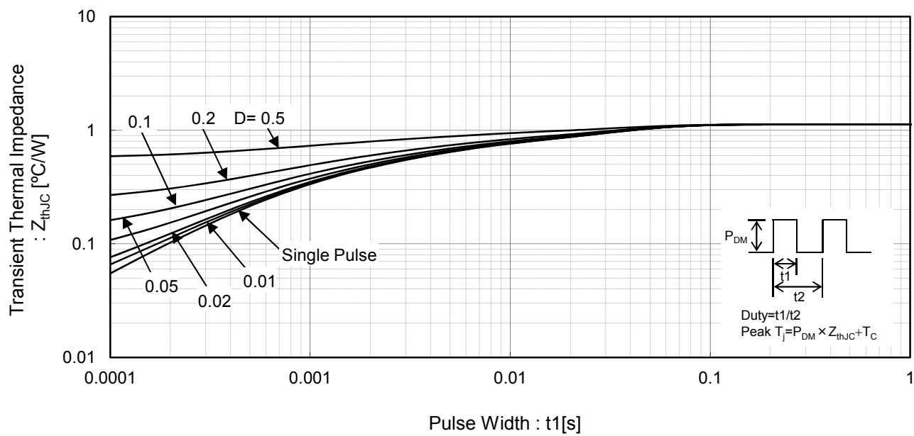
Fig.21 IGBT Transient Thermal Impedance
