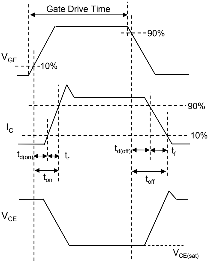
Fig.24 Inductive Load Waveform
