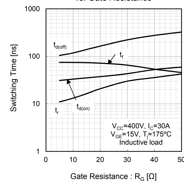
Fig.12 Typical Switching Time vs. Gate Resistance
