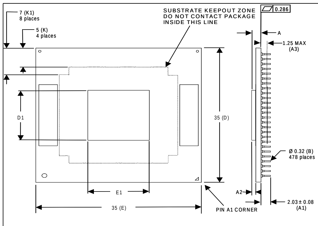
Figure 4-2. Micro-FCPGA Package - Top and Side Views
