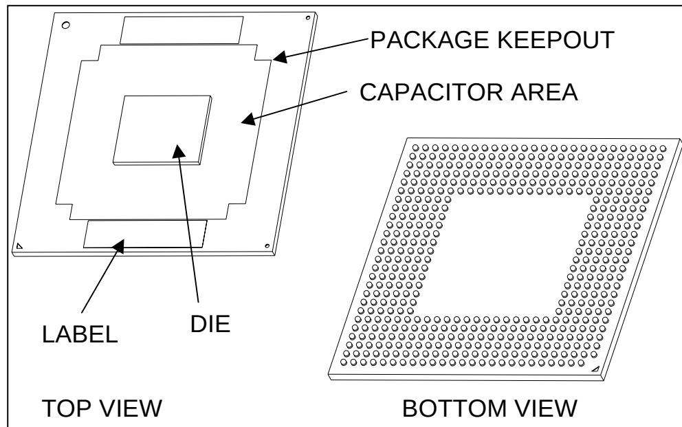
Figure 4-4. Micro-FCBGA Package Top and Bottom Isometric Views
