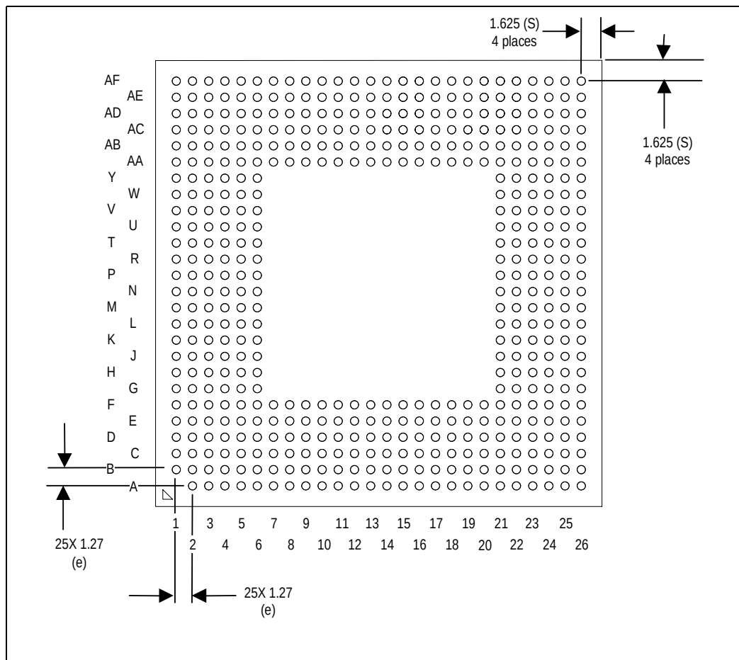
Figure 4-6. Micro-FCBGA Package Bottom View
