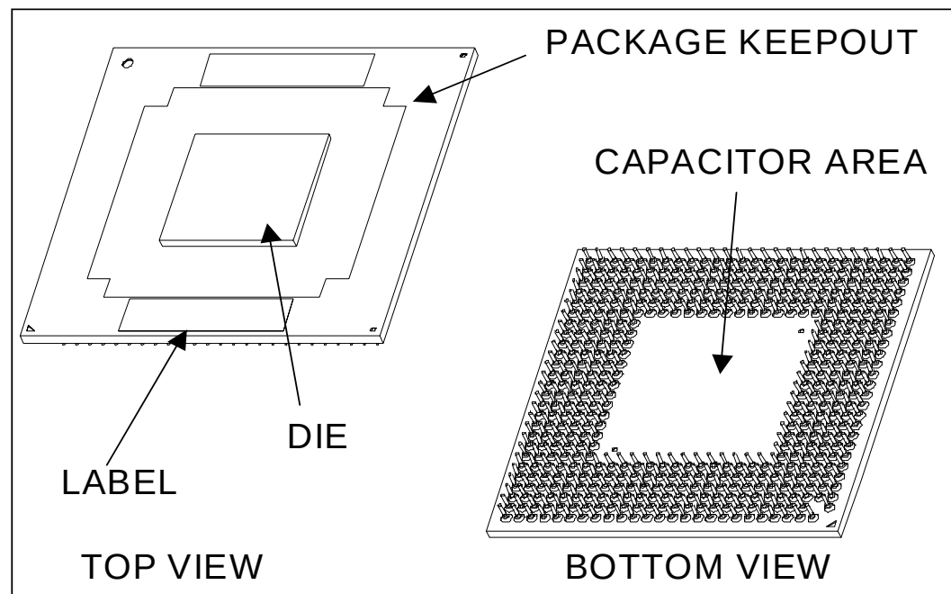
Figure 4-1. Micro-FCPGA Package Top and Bottom Isometric Views
