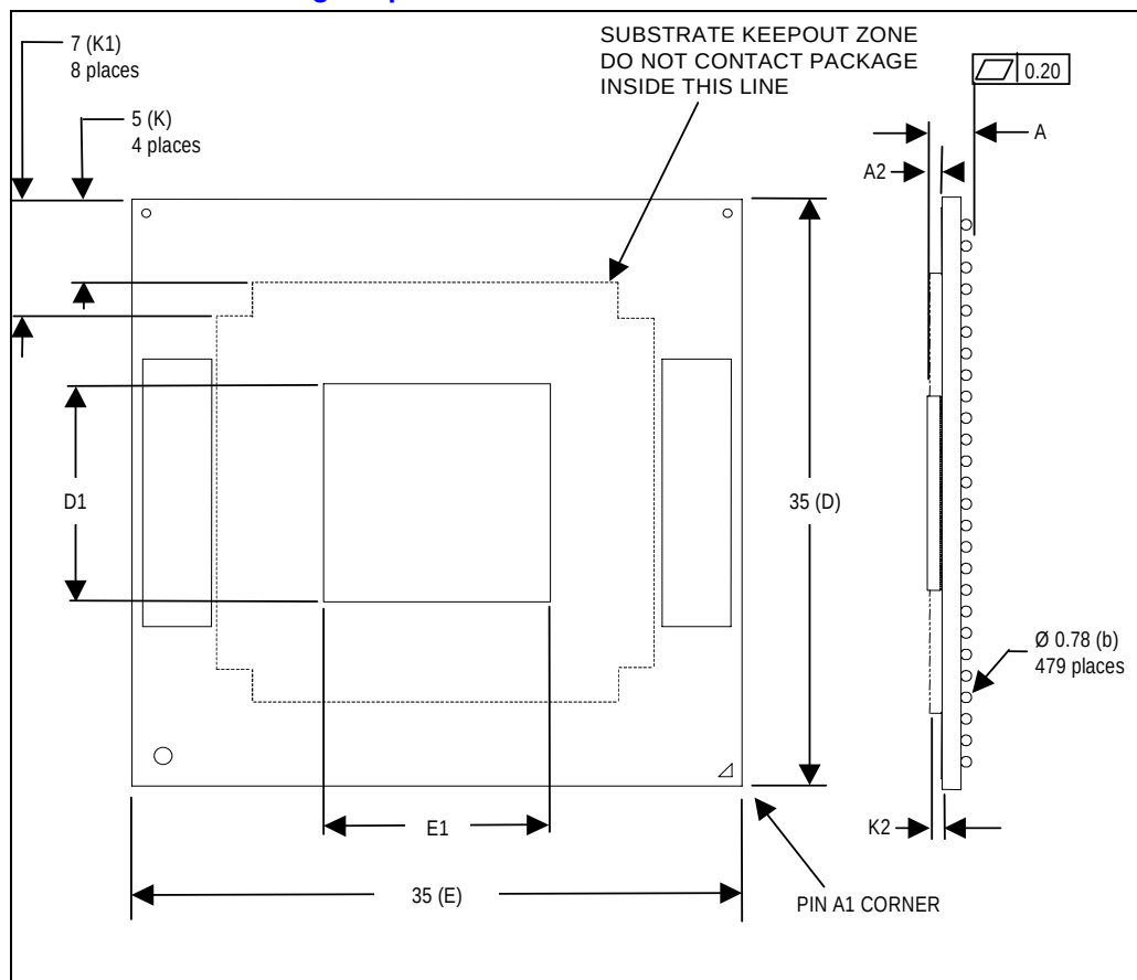
Figure 4-5. Micro-FCBGA Package Top and Side Views
