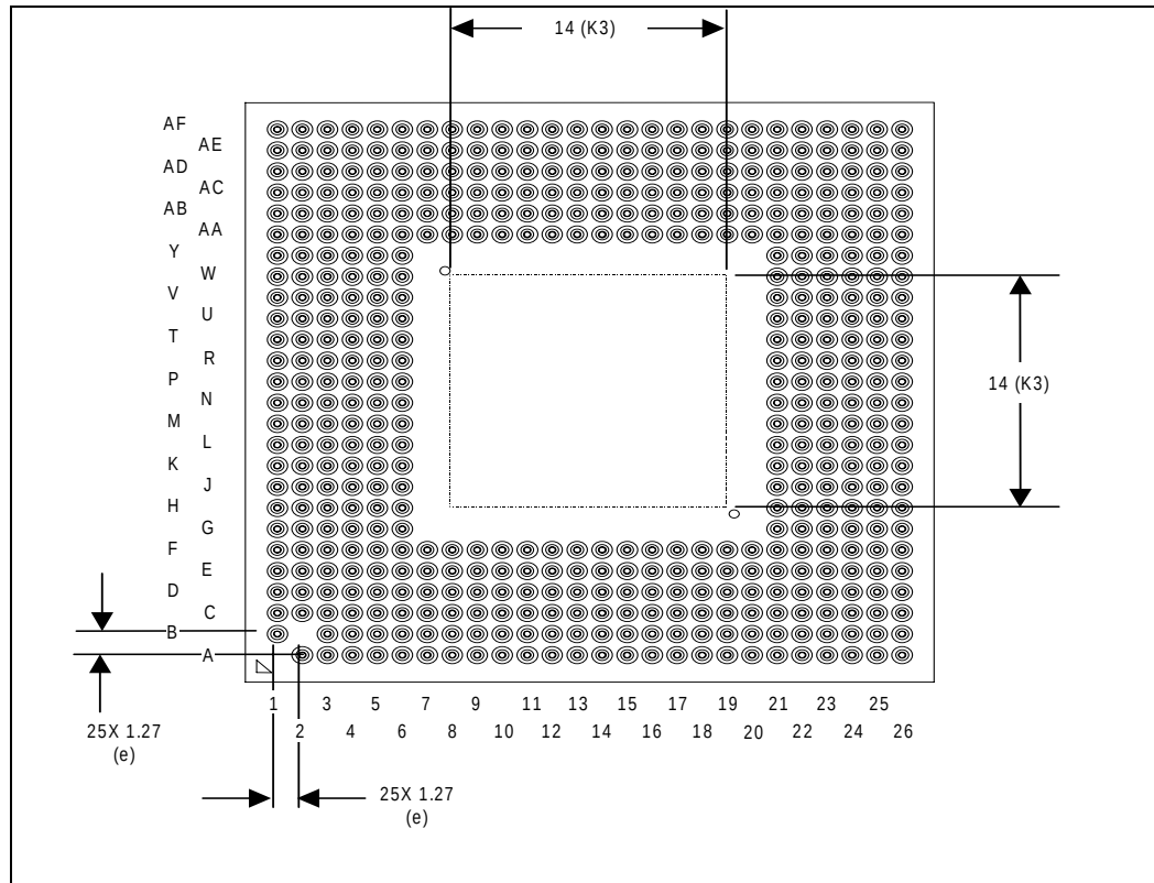
Figure 4-3. Micro-FCPGA Package - Bottom View
