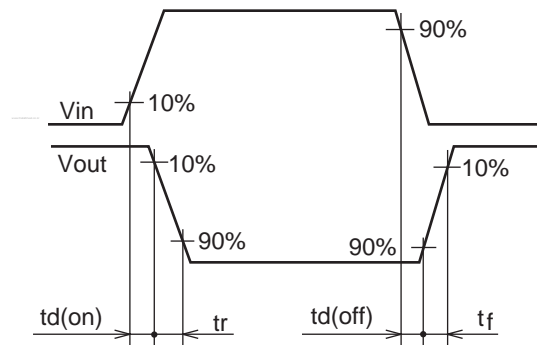
Waveform
