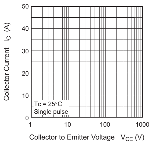
Turn-off Safe Operation Area
