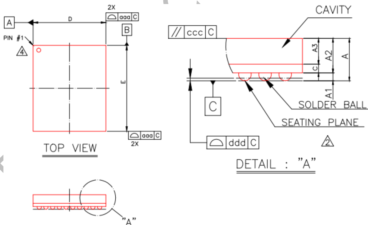
Fig.2-1 Package Top And Side View
