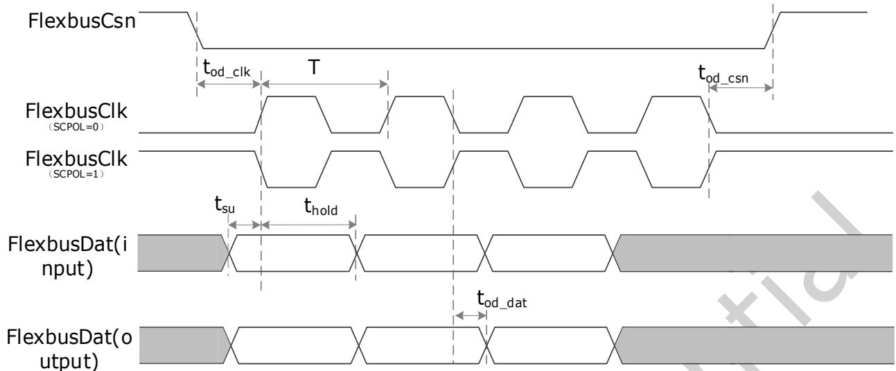
Fig.4-14 Flexbus interface master mode timing
