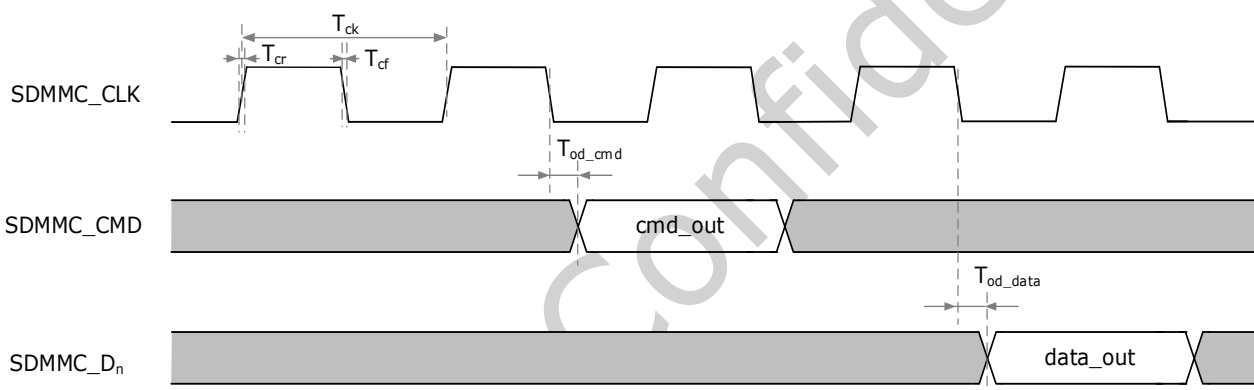
Fig.4-4 SDMMC output mode timing
