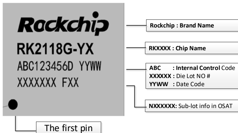
Fig.2-3 RK2118G-YX Package Definition
