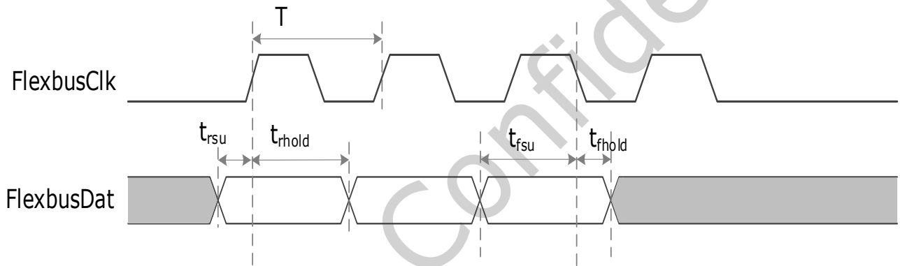
Fig.4-15 Flexbus interface slave mode timing
