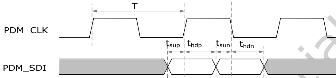
Fig.4-6 PDM interface timing
