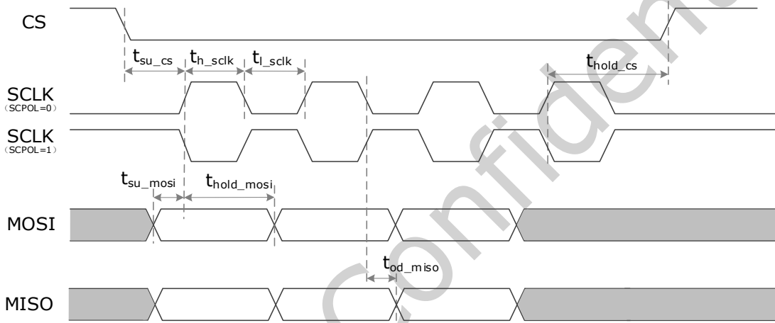
Fig.4-12 SPI interface slave mode timing
