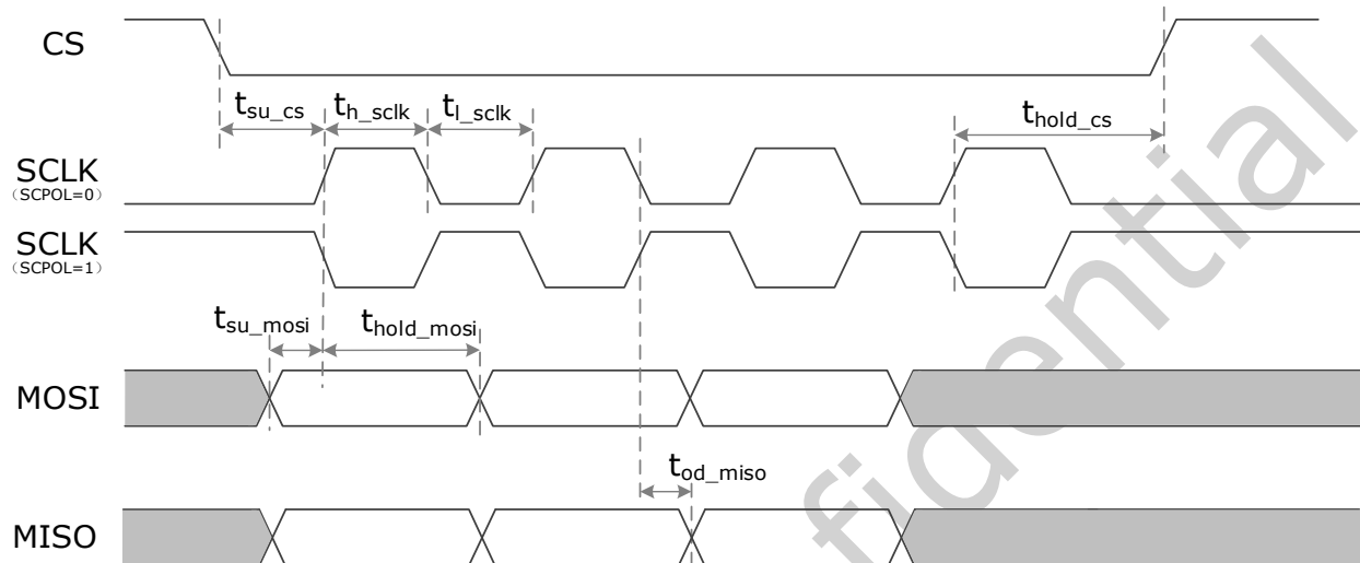
Fig.4-13 SPI2APB interface slave mode timing
