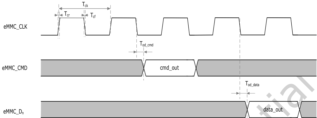
Fig.4-2 eMMC output mode timing
