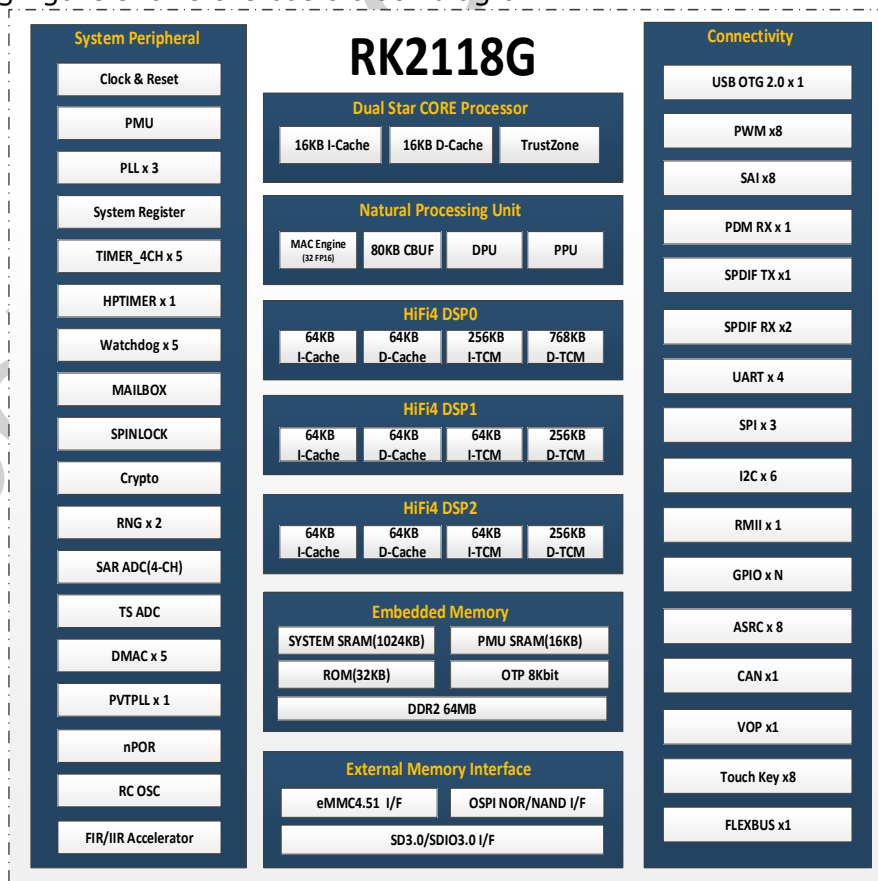
Fig.1-1 Block Diagram
