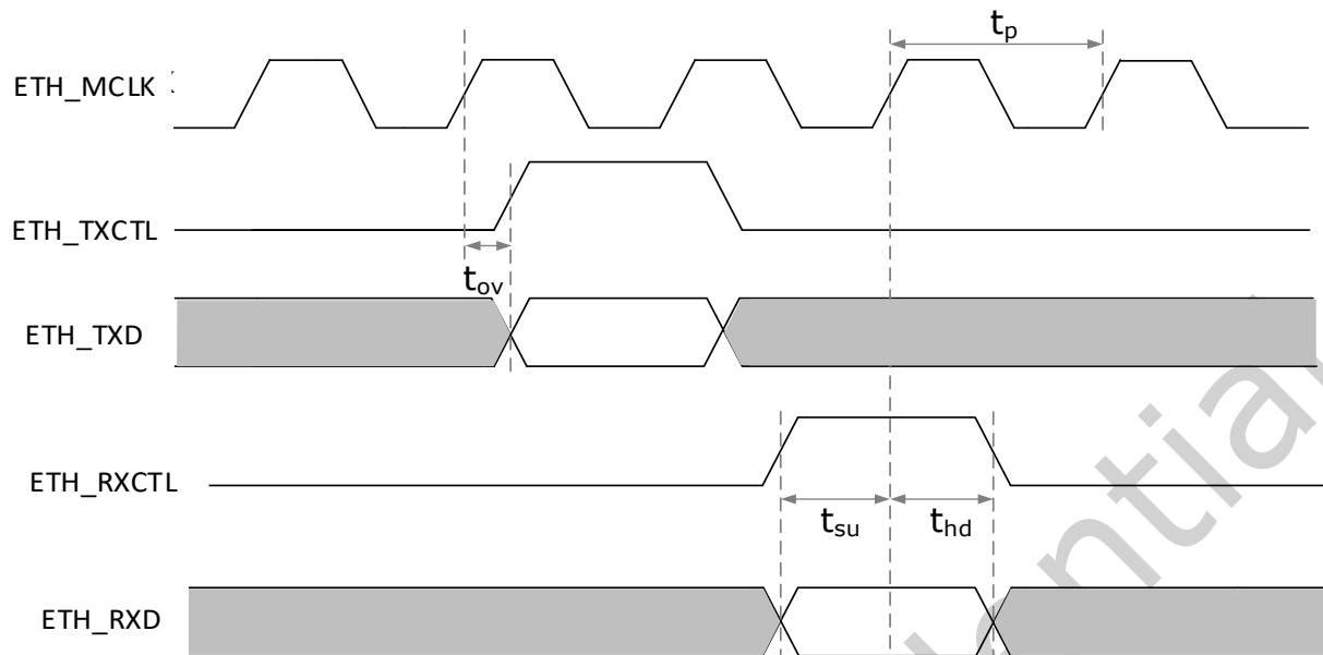
Fig.4-9 RMII interface timing
