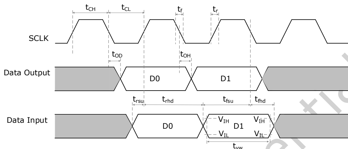
Fig.4-1 FSPI Interface Timing
