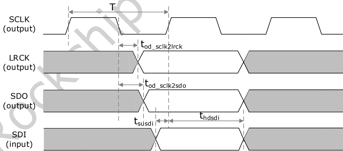
Fig.4-7 SAI interface master mode timing
