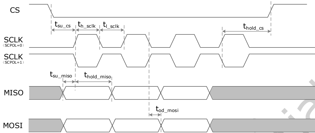
Fig.4-11 SPI interface master mode timing
