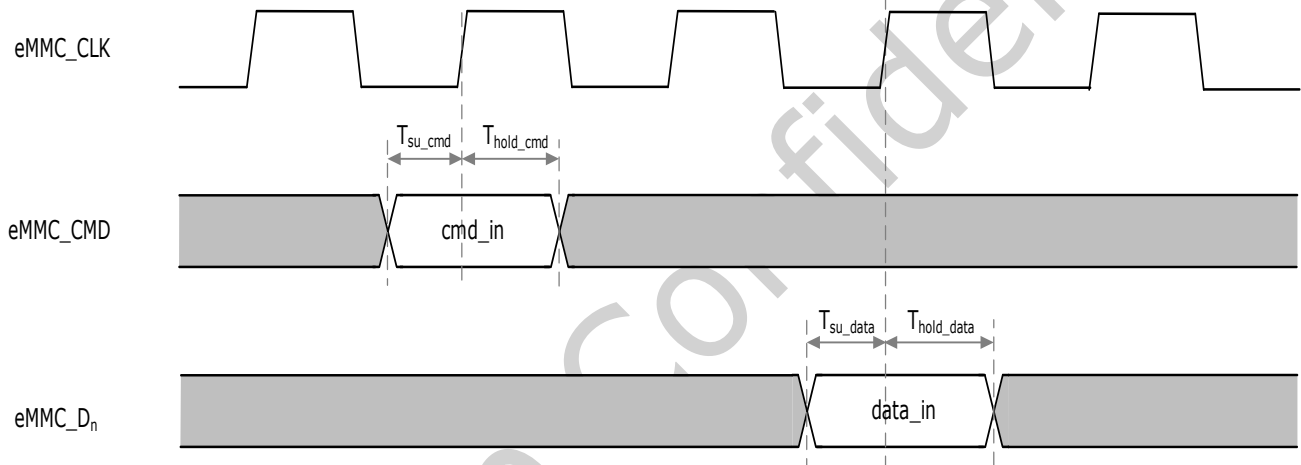
Fig.4-3 eMMC input mode timing
