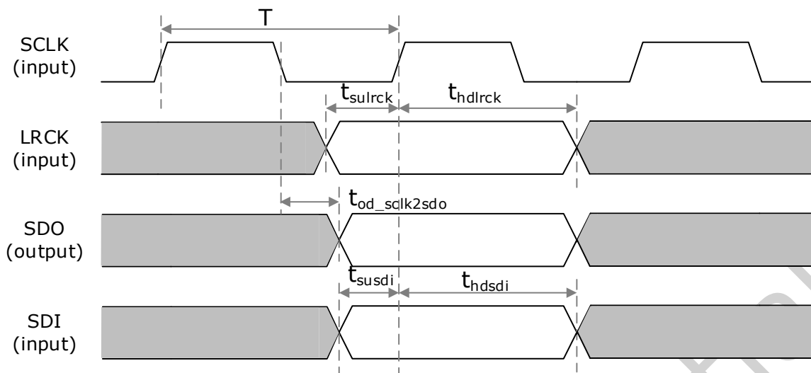
Fig.4-8 SAI interface Slave mode timing
