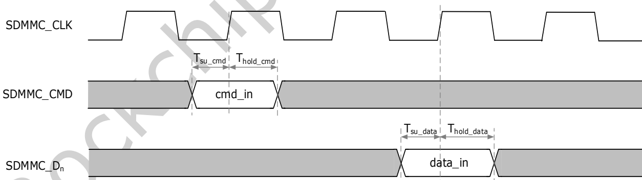
Fig.4-5 SDMMC input mode timing
