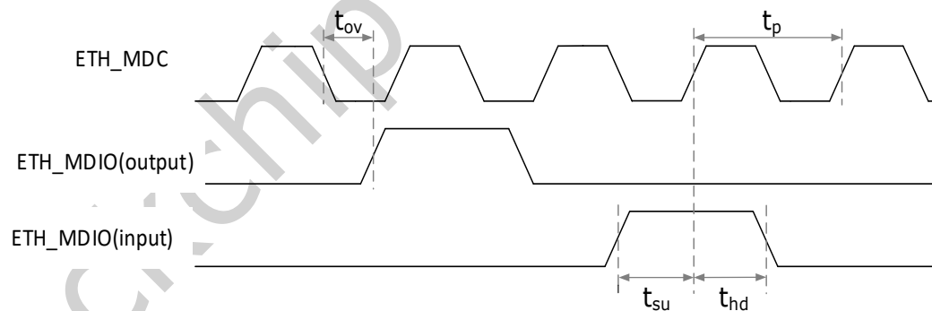
Fig.4-10 MDIO interface timing
