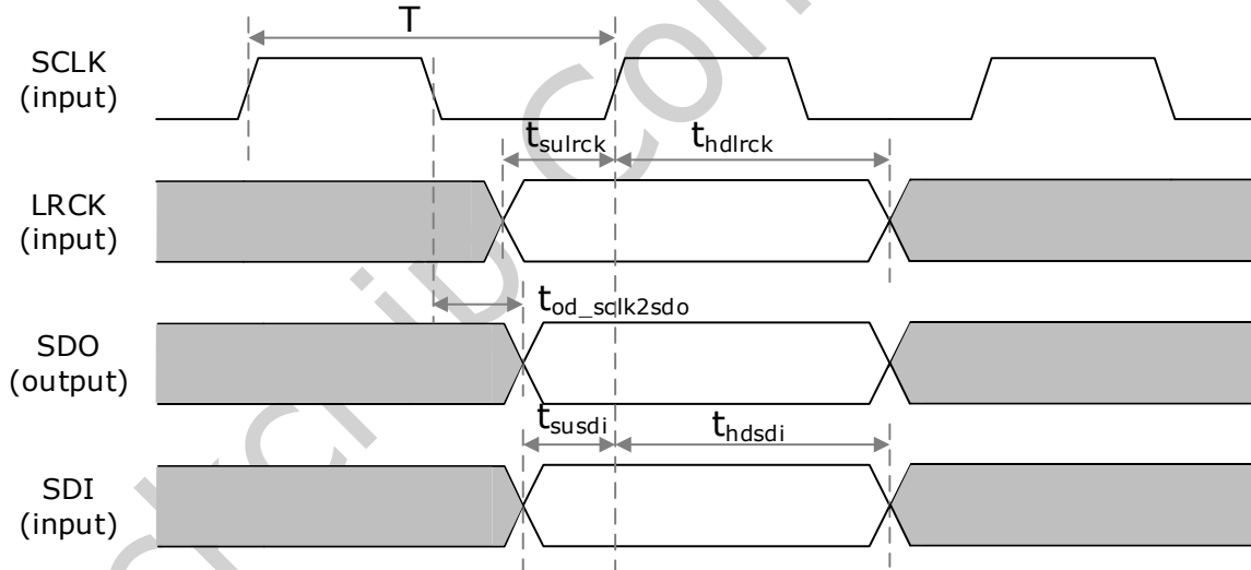
Fig.4-8 SAI interface Slave mode timing
