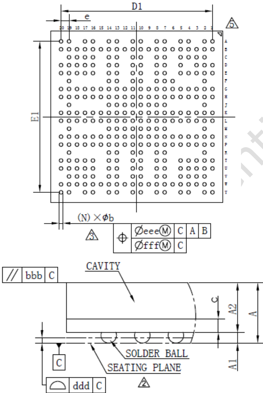
Fig. 2-1 RK3128H BGA316 Package Top View and bottom view
