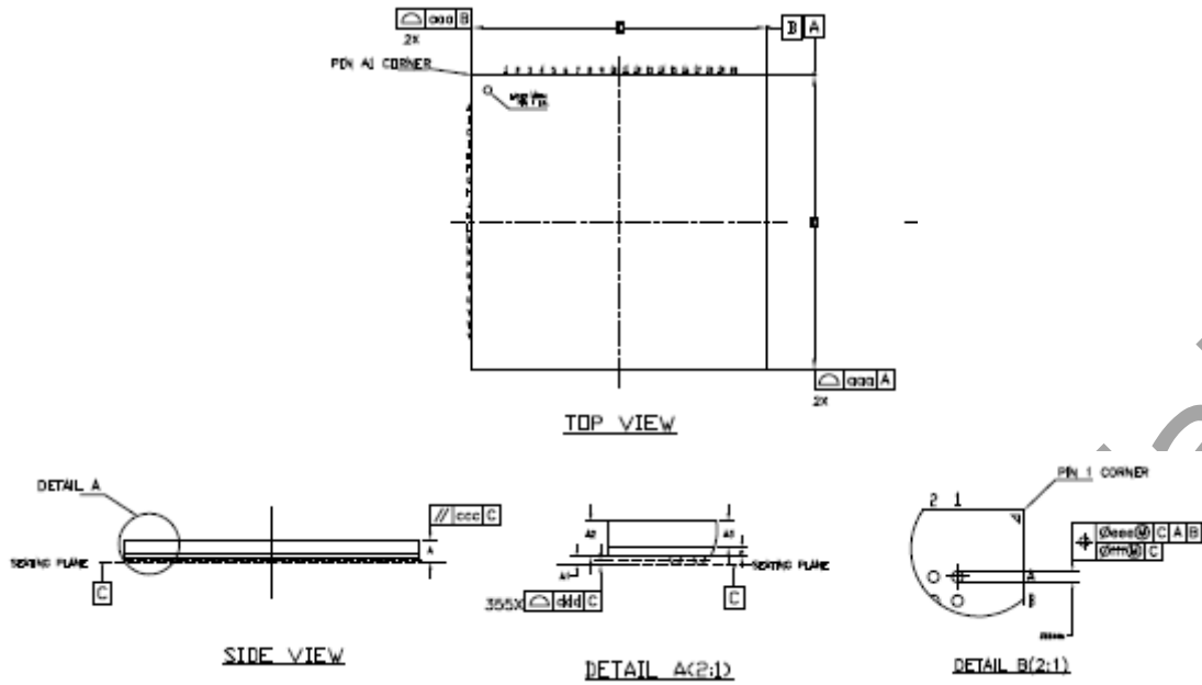
Fig.2-2 RK3308H3 Package Top View and Side View
