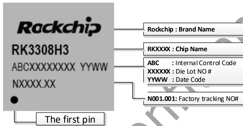
Fig.2-1 RK3308H3 Package definition
