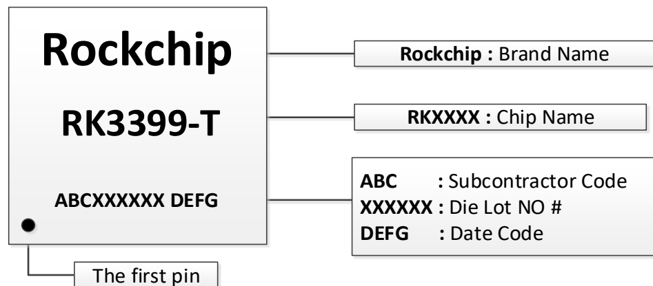
Fig. 2-1RK3399-T Top Marking
