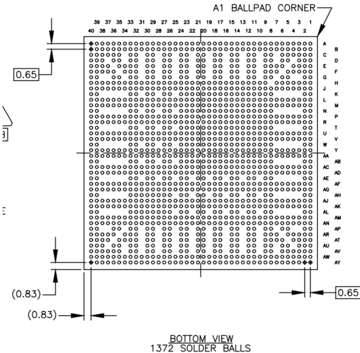
Fig. 2-3 Package Bottom View
