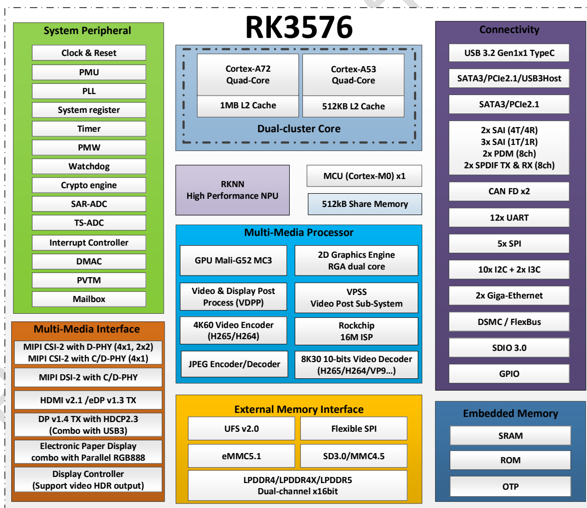
Fig.1-1 Block Diagram
