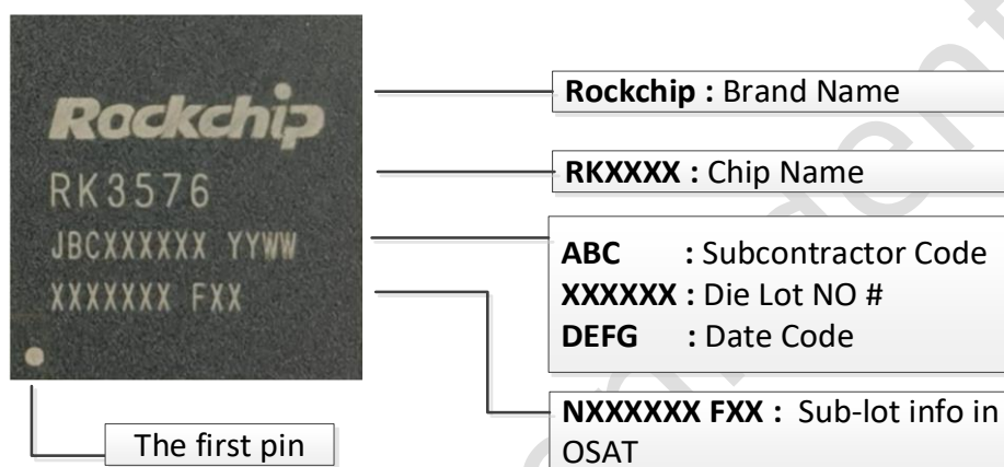
Fig.2-1 Package Definition
