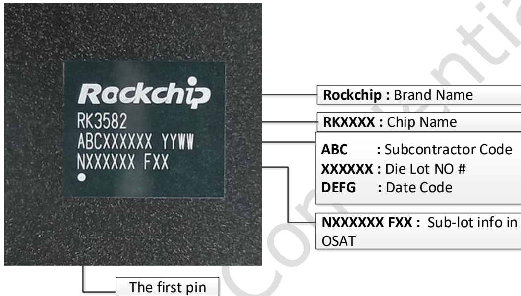
Fig.2-1 Package definition
