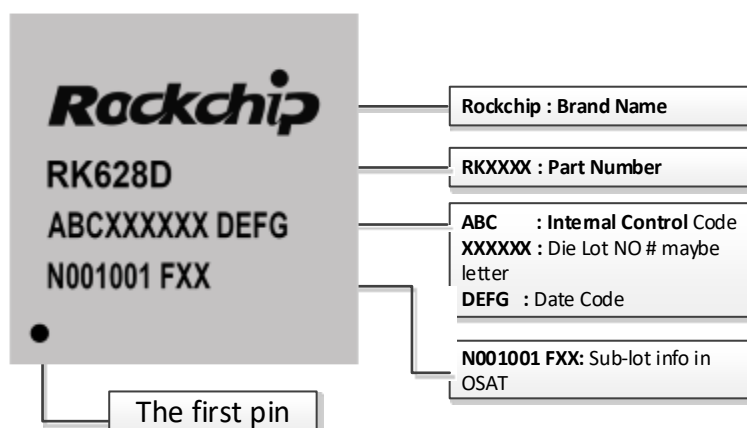
Fig. 2-1 Package Definition
