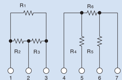
Example of custom circuit
