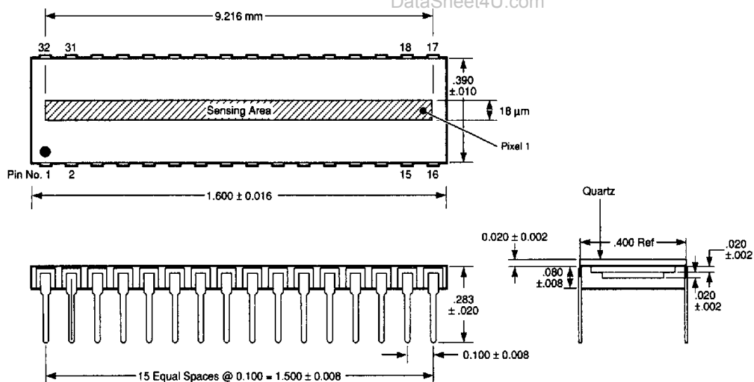
Packaging Dimensions RL1284D
