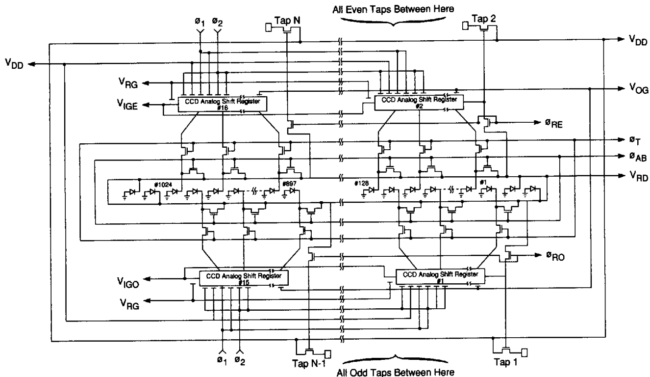
Figure 2. Schematic Diagram
