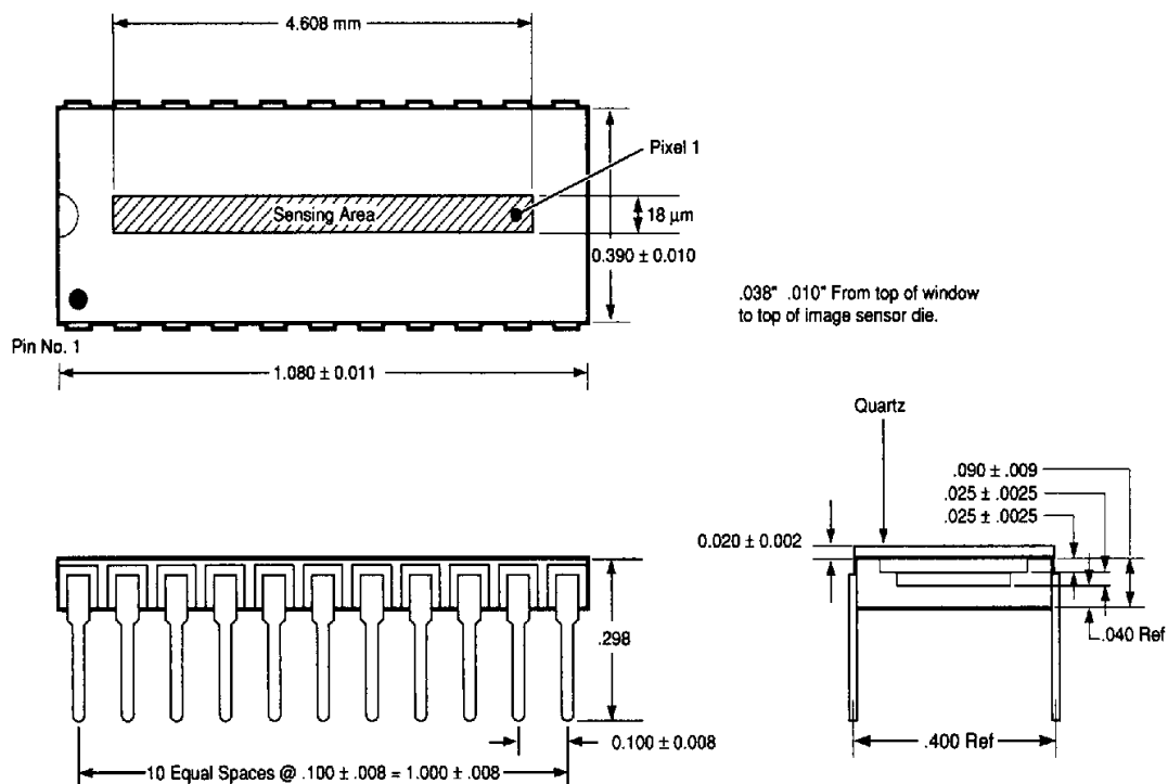
Packaging Dimensions RL1282D
